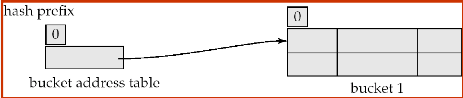
Initial Hash structure, bucket size = 2
